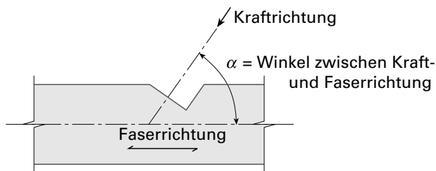
Figur 43 Schiefer Stoss
